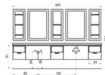
SCHEMA PER LAVELLO TONDO AD INCASSO TECHNICAL DRAWING FOR ROUND BUILT-IN SINK
