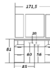
SCHEMA PER LAVELLO SOPRA PIANO TECHNICAL DRAWING FOR SINK ABOVE THE COUNTERTOP
